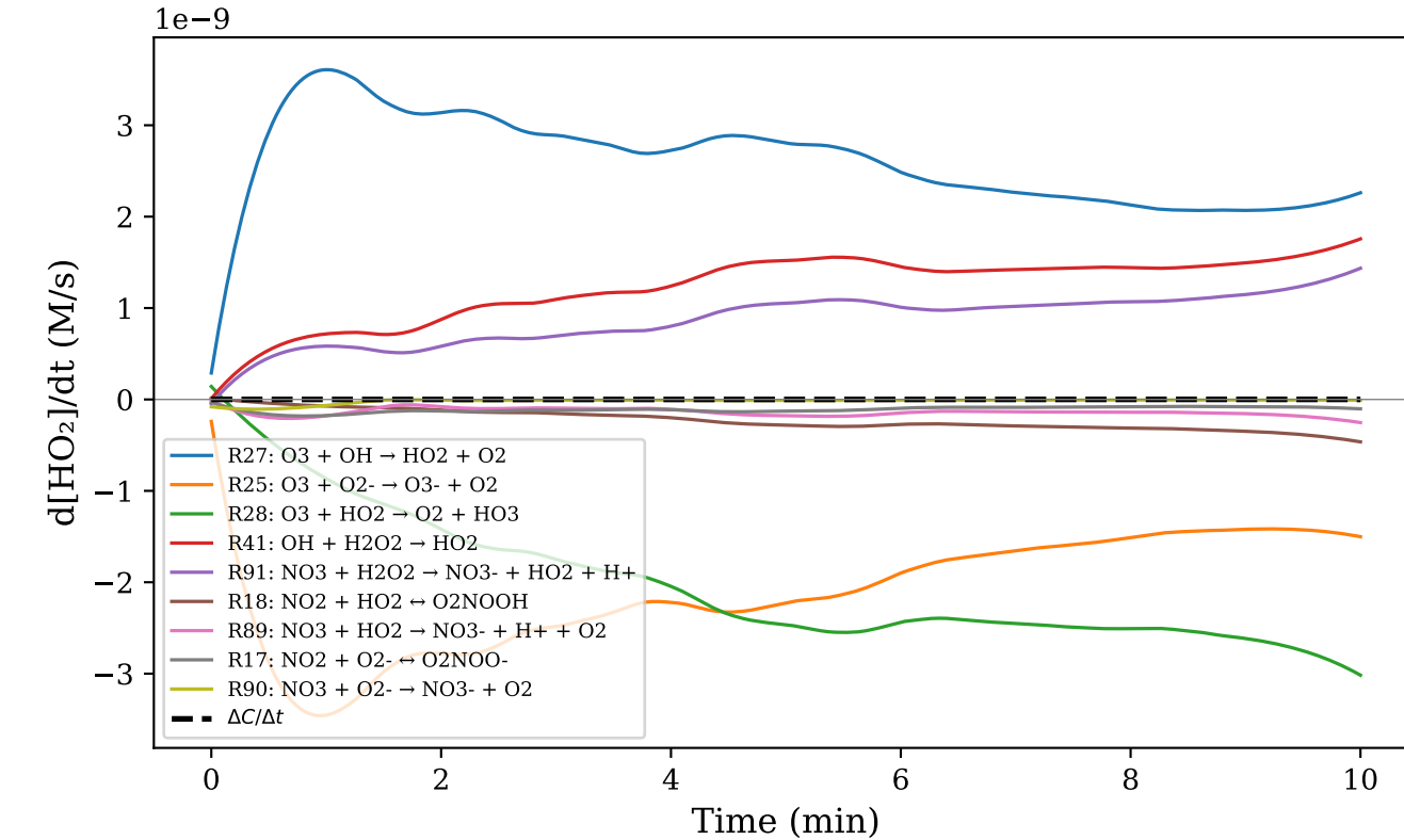
(c) HO 2 [final=179.90 pM]
